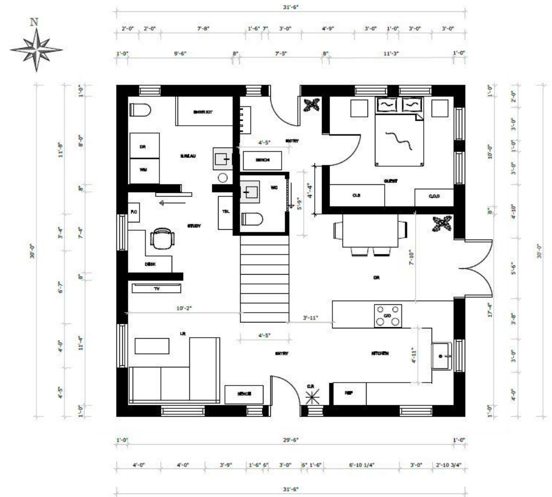
Final Floor Plan
